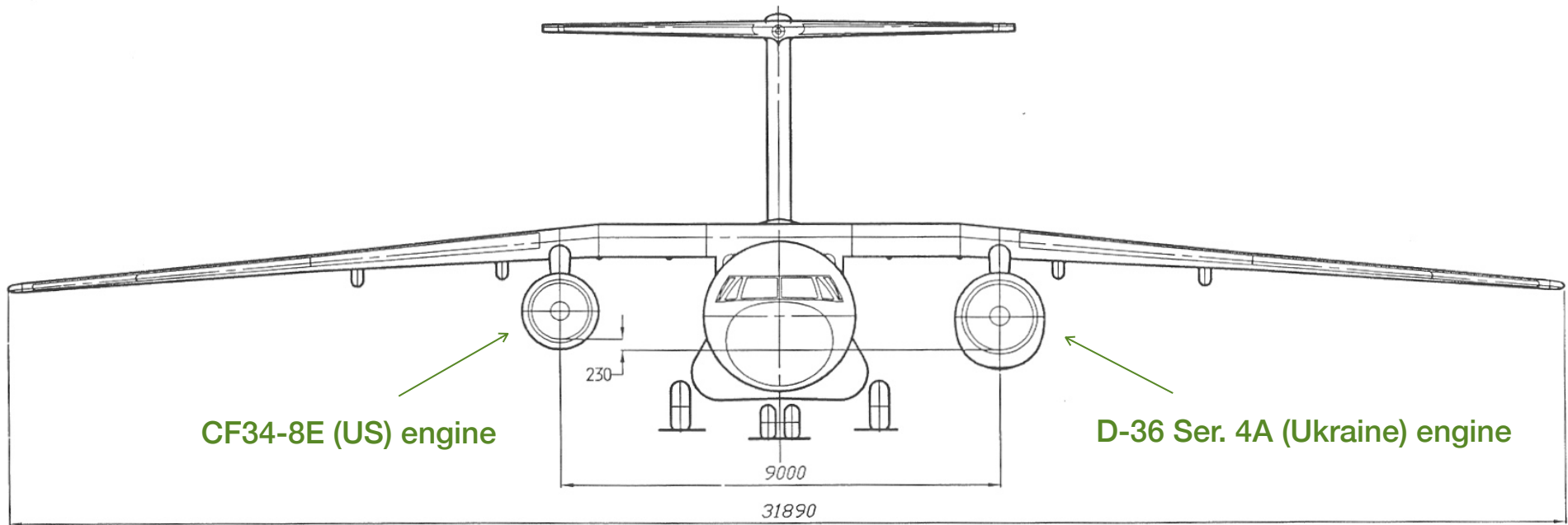
Antonov An-74TK-300 comparative concept with CF34-8E (US) & D-36 Ser. 4A (Ukraine)*
